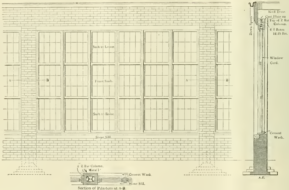
LAW'S PROPOSED NATURAL LIGHTING FOR ROUND HOUSES.
